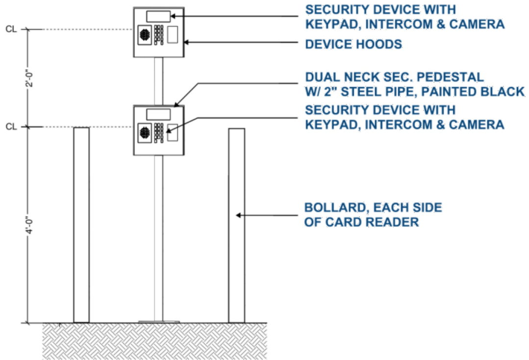
Standard Dual Neck Security Pedestal
