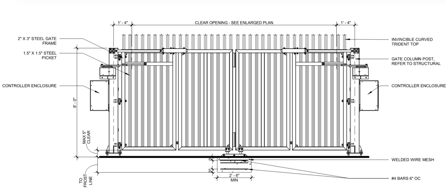
Standard Bi-Fold Gate Elevation
