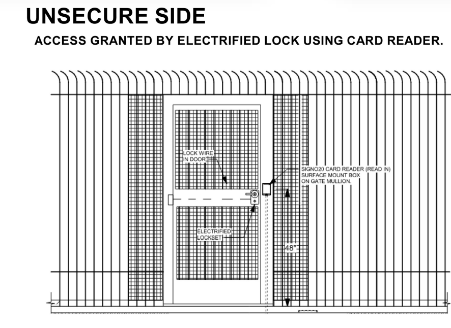
Standard Exterior Man-Gate Elevations
